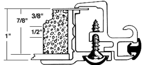
T6 Molded Trim Ring
