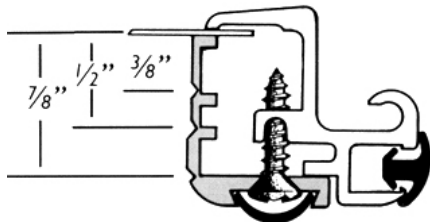
T5 Universal Trim Ring
